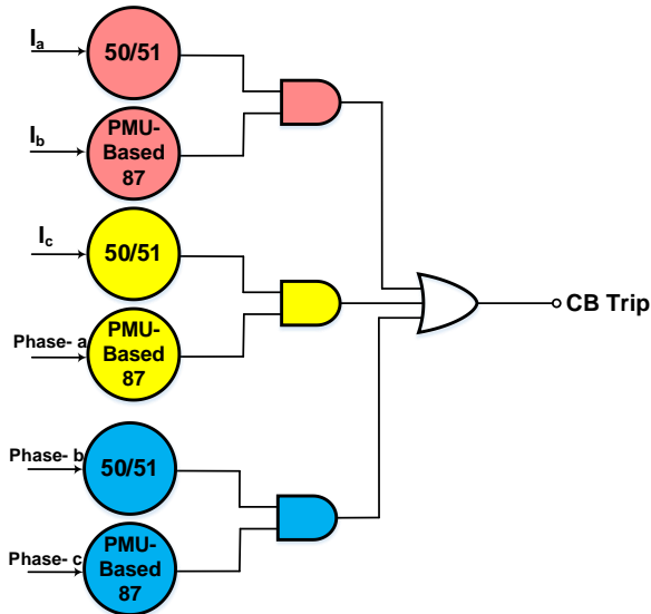
Figure 8: Protection logic of each DER.
