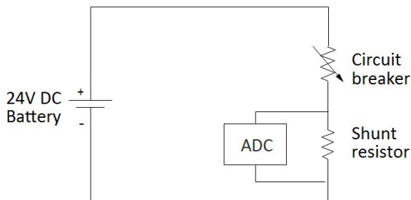
Fig. 1: Circuit diagram for measuring current using the new tool.
