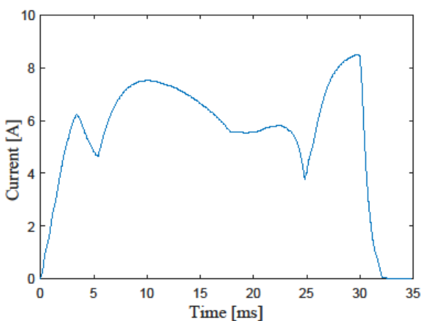
Fig.6 Trip current waveform during relay contact problem. The current rise during the time period T1 is not linear as compared to Fig. 4.
