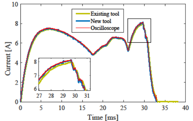
Fig. 3: Measurements recorded near trip coil. The inset shows the small differences in waveforms.
