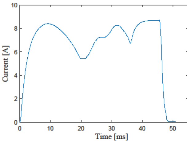
Fig.5 Trip current waveform during roller bearing problem. The pattern and duration of the time period T2 differs when compared to Fig. 4.
