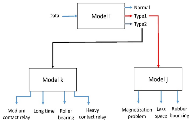
Fig9. Automated two step analysis with three models i, j and k.
