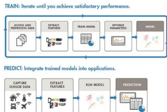
Fig.8 Machine Learning Process [5]
