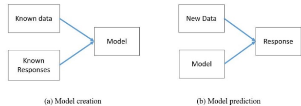
Fig.7 Supervised Machine Learning
