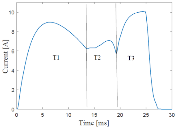
Fig.4 Trip current pattern under normal operation of CB.
