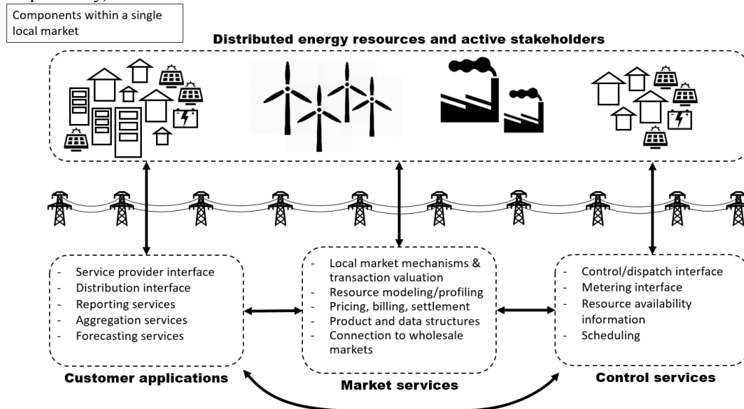
Figure 2 - Three innovation areas of DOMINOES project: market services, control services and customer applications.
