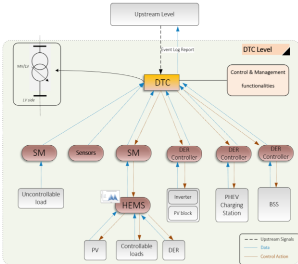
Fig. 1 Conceptual framework based on centralized management - substation centered approach.
