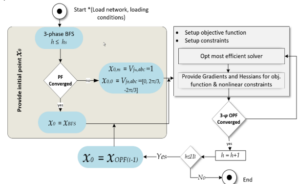
Fig. 2 Algorithm for the scheduling of operation, describing the important steps for the optimization stages.
