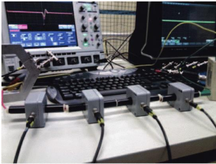
Figure 4. Directional calibration of HFCTs.
