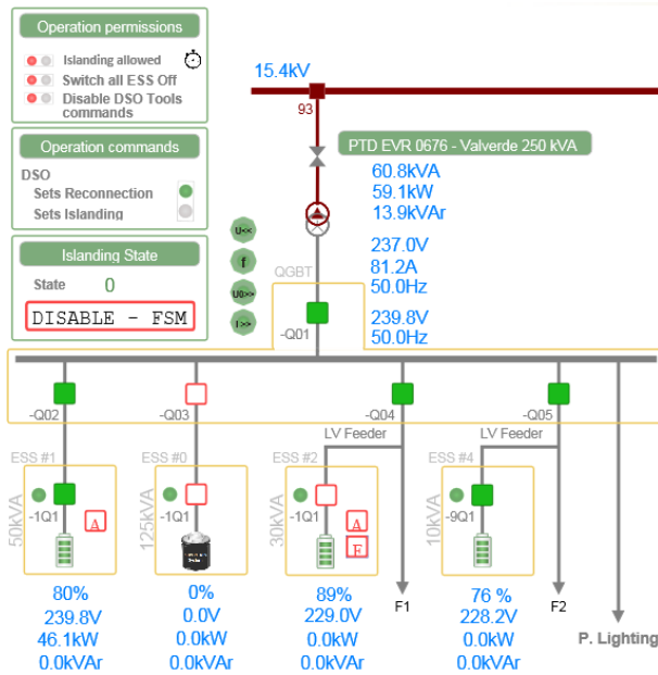
Figure 1 - System Architecture
